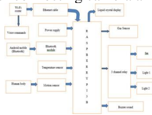
Fig 2:- Block Diagram
