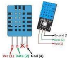
Fig 4:- Temperature Sensor
