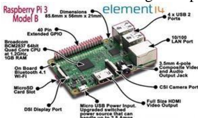
Fig 1:- Diagram of Raspberry Pi 3B
